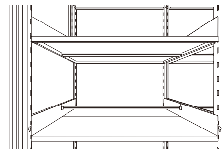
透視圖 2 shelves share the same shelf trays
